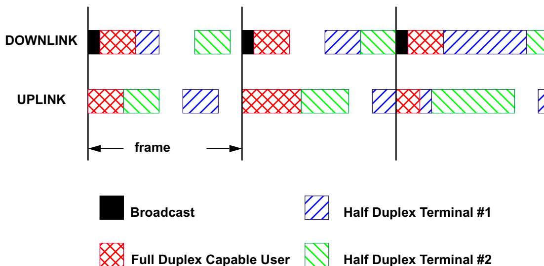
FIGURE 2. Example of Burst FDD Bandwidth Allocation
