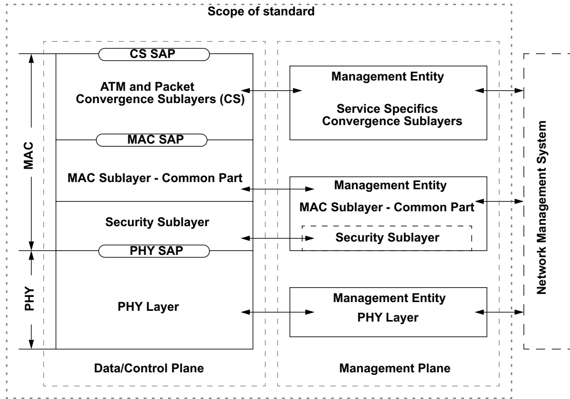
FIGURE 1. IEEE 802.16 Reference Model and Protocol Stack
