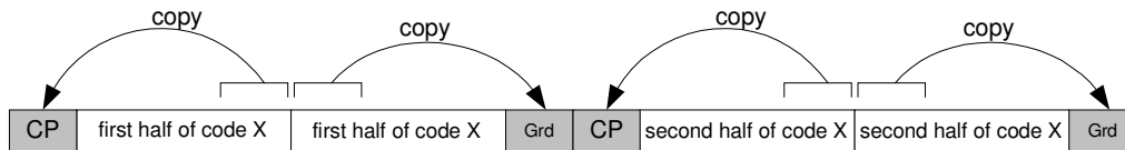
Figure 240a - Initial-ranging transmission for OFDMA, using a single code over four consecutive symbols
