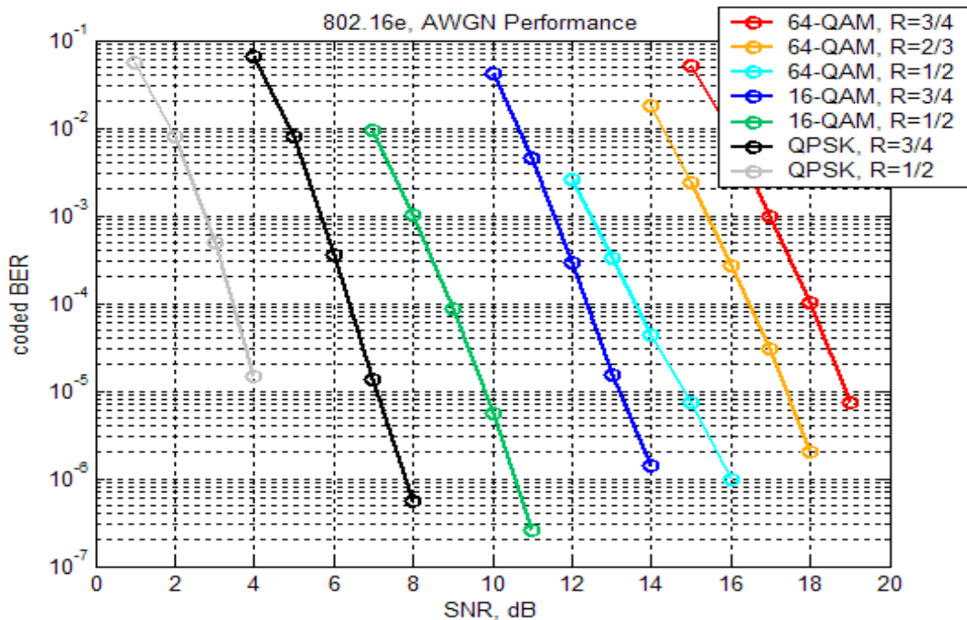
Figure 1: Theoretical BER for OFDMA in AWGN
