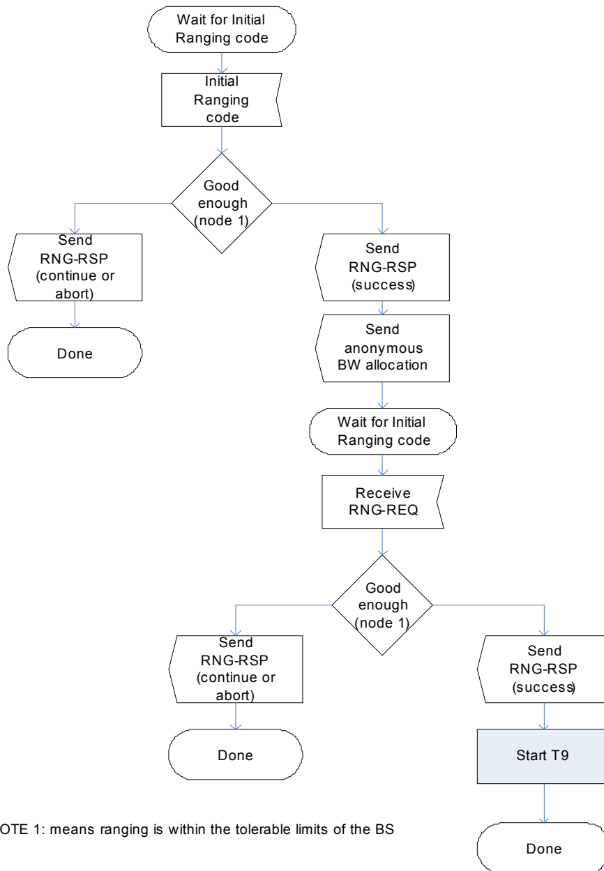
Figure 87 CDMA Initial Ranging -- BS
