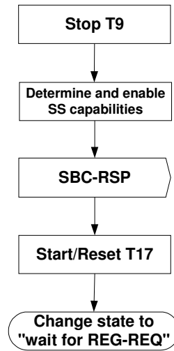
Figure 67-Handling SBC-REQ
