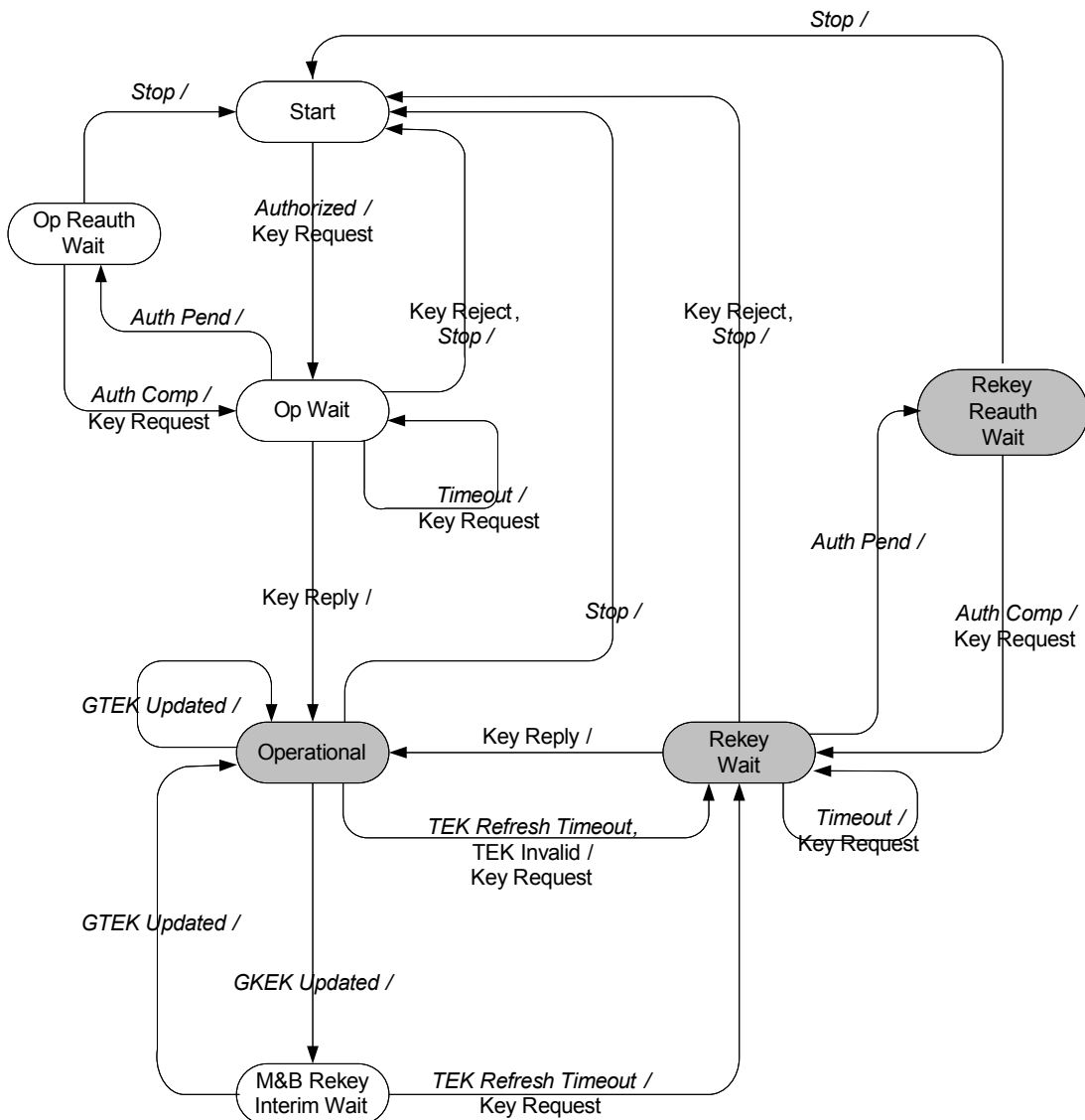
Figure 4-131—TEK state machine flow diagram
